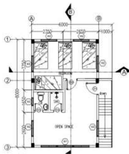
SECOND FLOOR PLAN SCALE 1:50M
