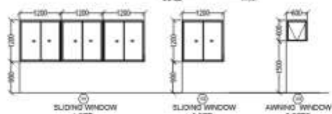
SCHEDULE OF DOORS & WINDOW SCALE 1:50M
