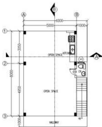
GROUND FLOOR PLAN SCALE 1:50M
