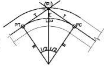
TYPICAL HORIZONTAL CURVE D 0-2 SCALE I/TB
