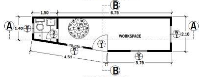
FLOOR PLAN LAYOUT SCALE: 1:800 (M/S)
