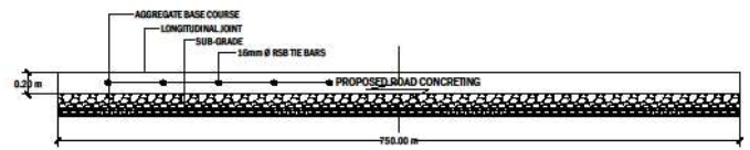
SECTION - A
