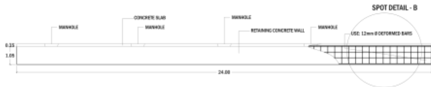
SIDE ELEVATION SCALE: 1:48 MTS.
