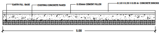
CROSS - SECTION - A SCALE: 1:145 MRS.
