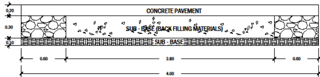
LATTITUDINAL SECTION - A SCALE: 1:80 MTS.
