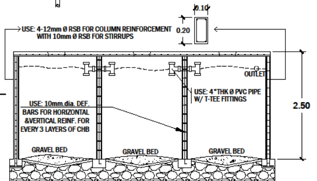
SEPTIC VAULT DETAIL
