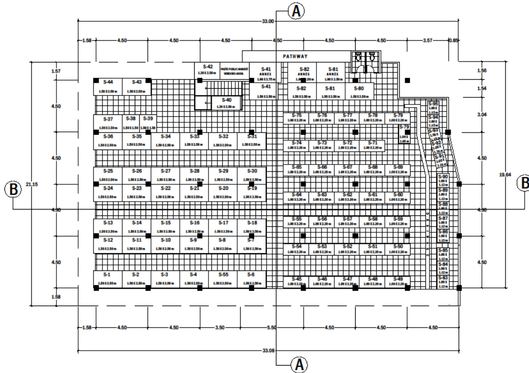
FLOOR PLAN LAYOUT SCALE: 1:250 MTS.
