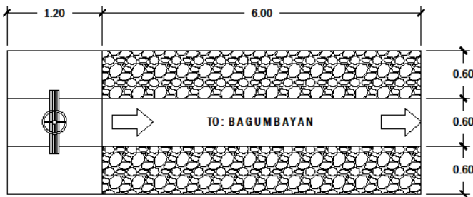
FLOOD GATE - 2 PLAN SCALE: 1:20 MTS.
