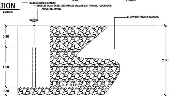
SIDE ELEVATION SCALE: 1:20 MTS.
