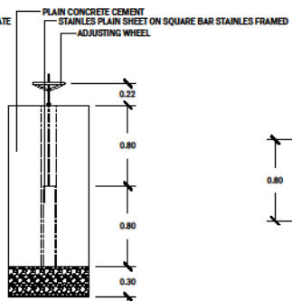
SIDE ELEVATION SCALE: 1:20 MTS.
