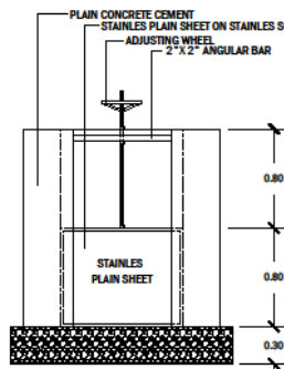
FRONT ELEVATION SCALE: 1:20 MTS.
