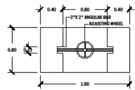
FLOOD GATE - 1 PLAN SCALE: 1:20 MTS.
