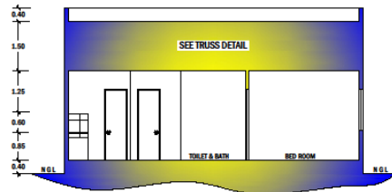
LATTITUDINAL CROSS SECTION - B SCALE: 1:450 MTS.
