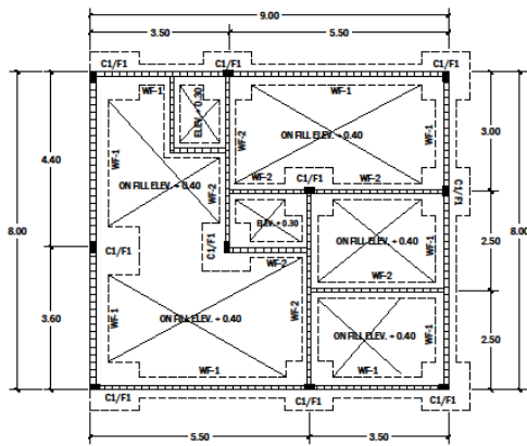
FOUNDATION PLAN LAYOUT SCALE: 1:450 MTS.
