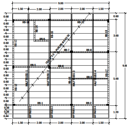
ROOF FRAMING PLAN LAYOUT SCALE: 1:450 MTS.
