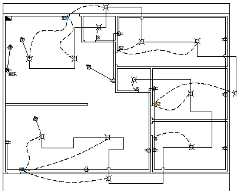
ELECTRICAL LAYOUT SCALE: 1:400 MTS.
