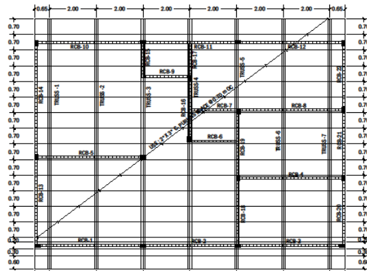
ROOF FRAMING PLAN LAYOUT SCALE: 1:400 MRS.
