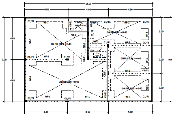
FOUNDATION PLAN LAYOUT SCALE: 1:400 MRS.
